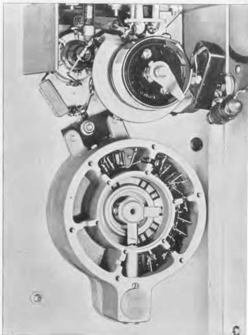
FIGURE 5. View of the attenuator with the cover of the multiplier housing removed. At the top is the Ayerton-Perry-wound output control.
