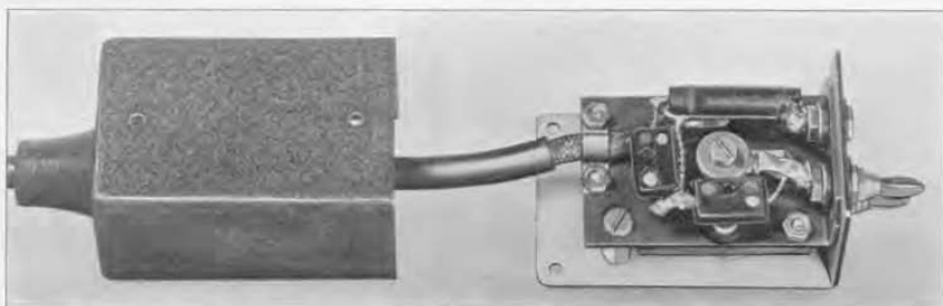
FIGURE 6. View of the cable terminating unit removed from its housing.
